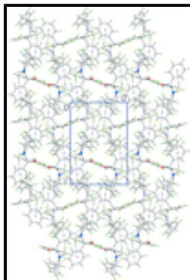
Fig. 2. A view in projection down the b axis of the unit-cell contents for (I). The C—H... \pi interactions are shown as purple dashed lines.
